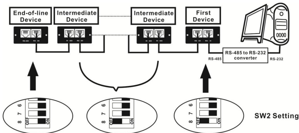
End-of-line Device
